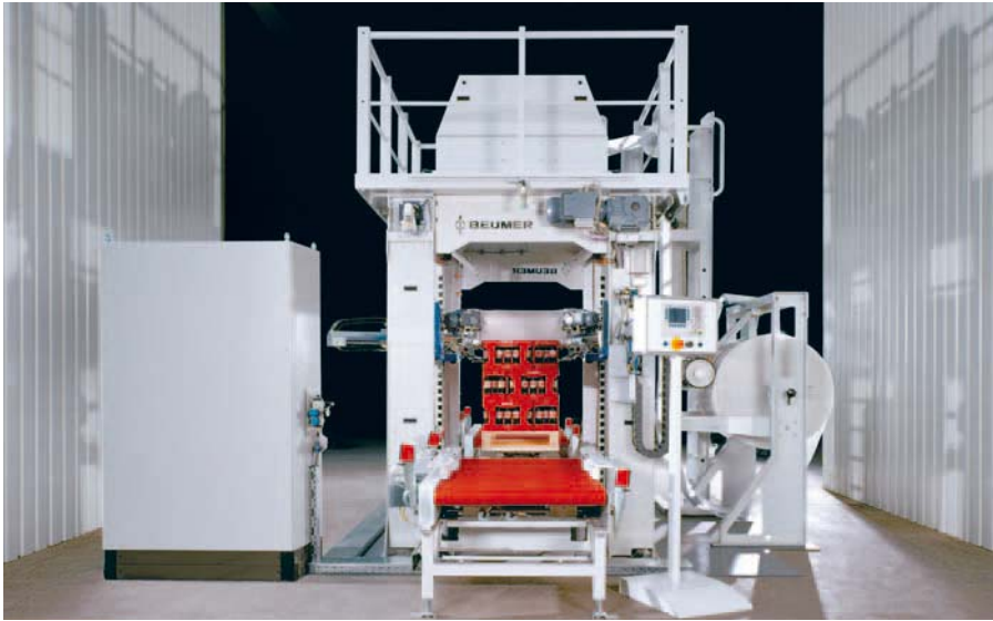
The BEUMER stretch hood® system does not shrink the film.
